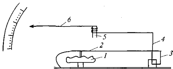
1.2-rasm. Metall barometr:
