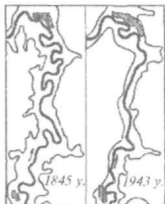
13.10-rasm. Daryo o'zani egriligining vaqt maboynida o'zgarishi (1845—1943).
