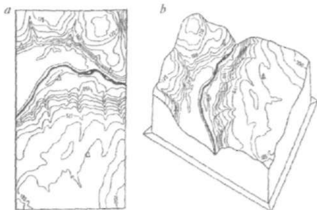
4.5-rasm. Joyning relief kartasi (a), uning gorizontallarda avtomatik ravishda tuzilgan blok-diagrammasi (b).
