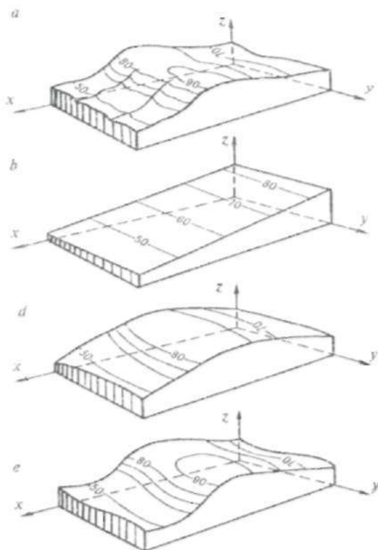
12.15-rasm. Yuzalarni approssimasiyalash (yaqinlashtirish).
