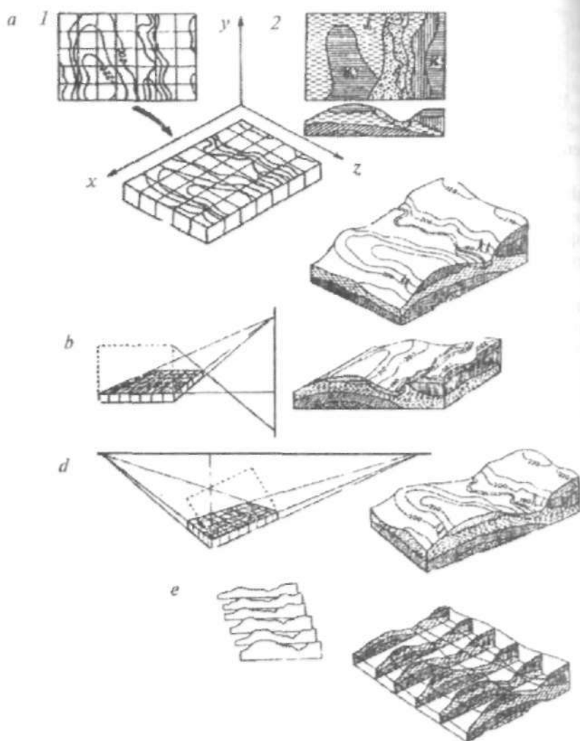
12.8-rasm. Blok-diagrammalar.
