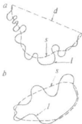
12.14-rasm. Egri chiziqlarning buralmaligini aniqlash.
